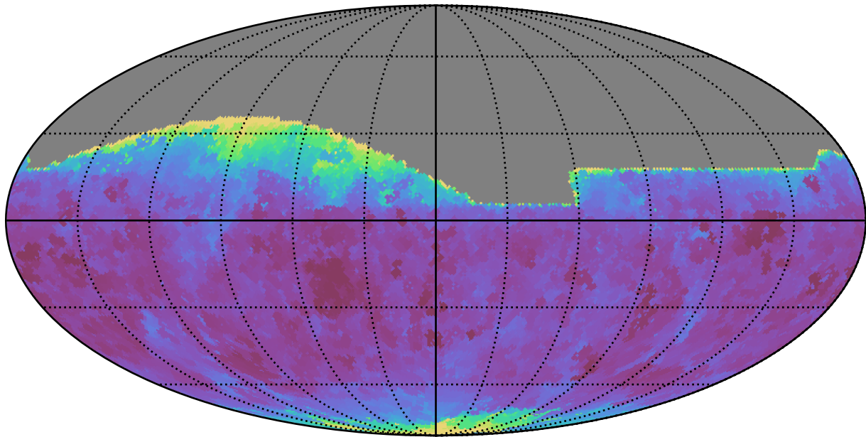
weather_cloudso14v3.4_10yrs All sky r band: Min seeingEff
