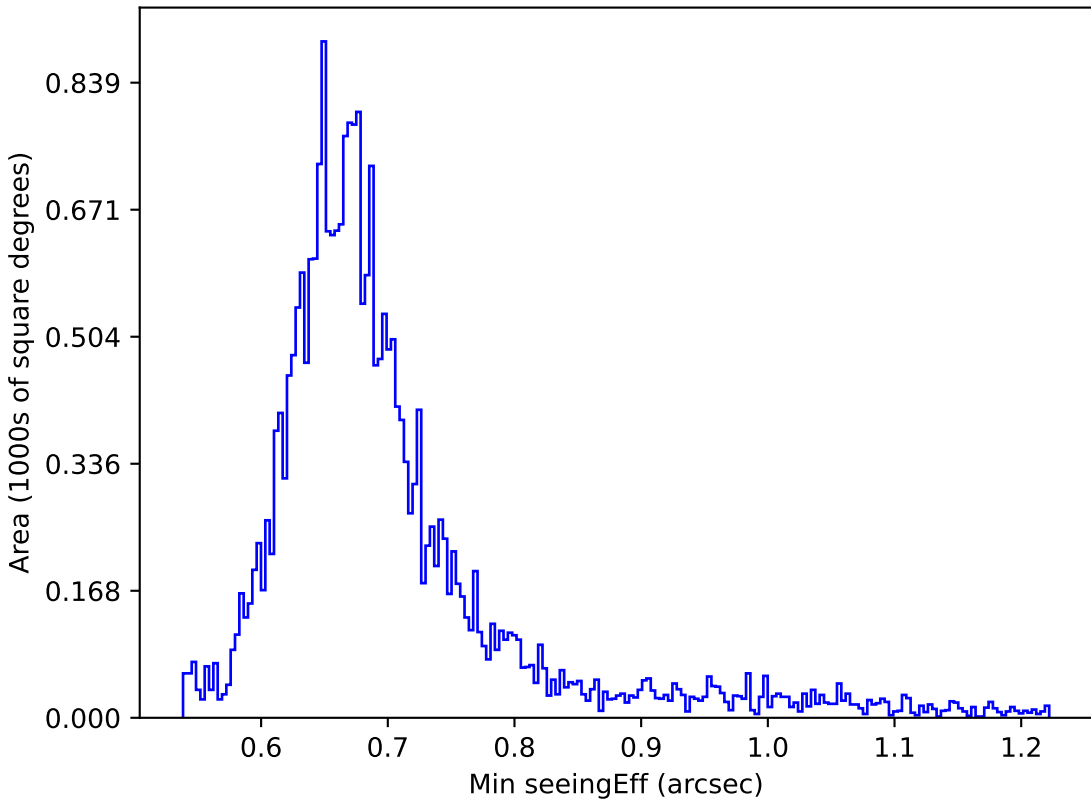
weather_cloudso14v3.4_10yrs All sky g band: Min seeingEff
