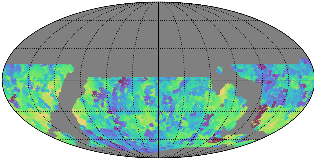
weather_cloudso14v3.4_10yrs WFD all bands: Min saturation_mag
