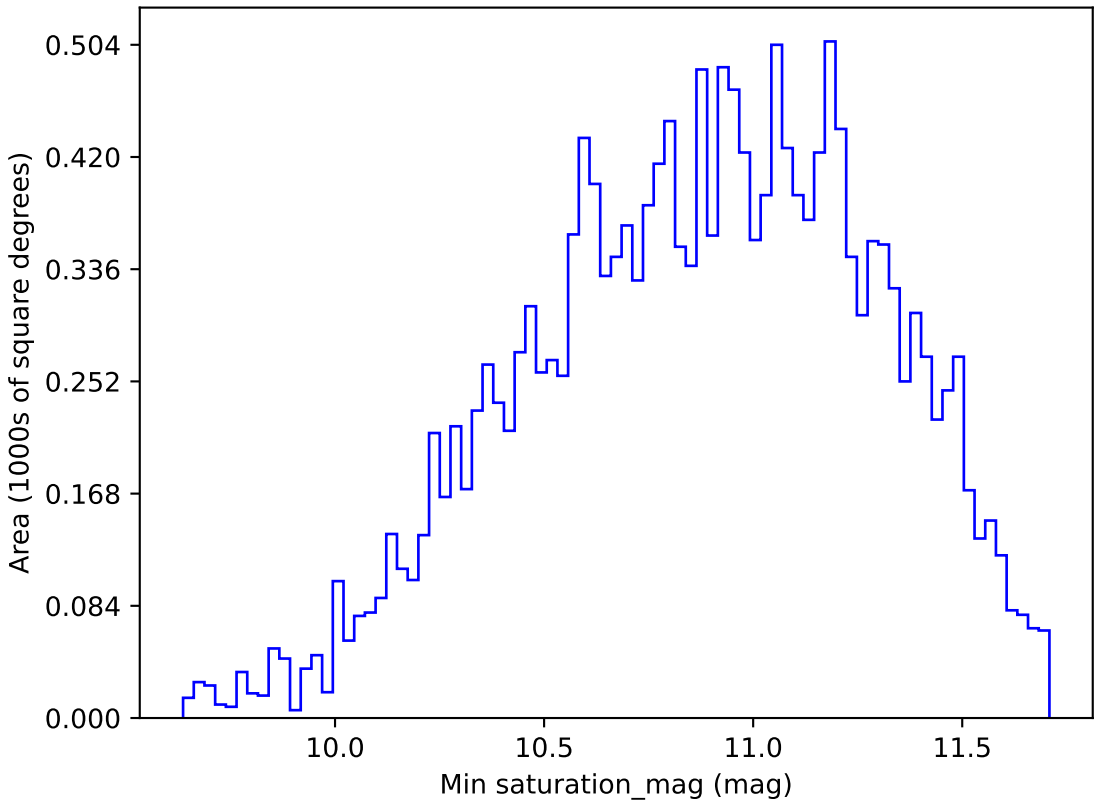
weather_cloudso14v3.4_10yrs WFD all bands: Min saturation_mag
