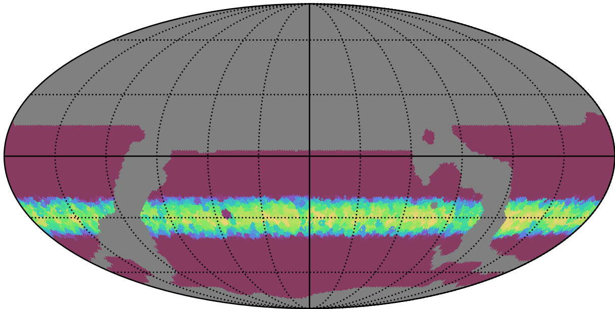
weather_cloudso14v3.4_10yrs WFD all bands: Min normairmass
