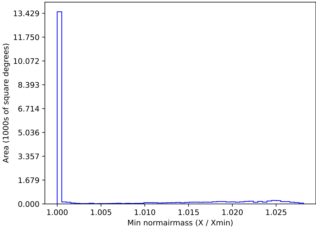
weather_cloudso14v3.4_10yrs WFD all bands: Min normairmass
