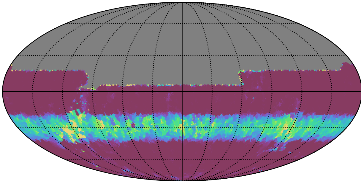
weather_cloudso14v3.4_10yrs All sky u band: Min normairmass
