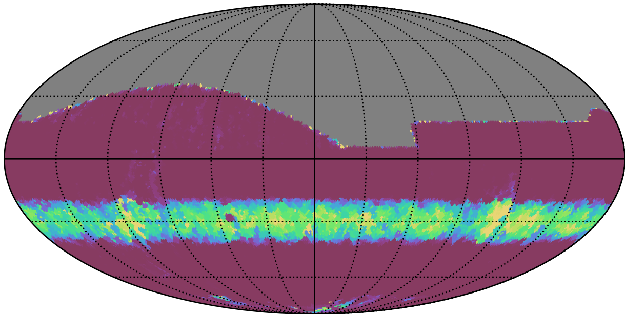
weather_cloudso14v3.4_10yrs All sky r band: Min normairmass
