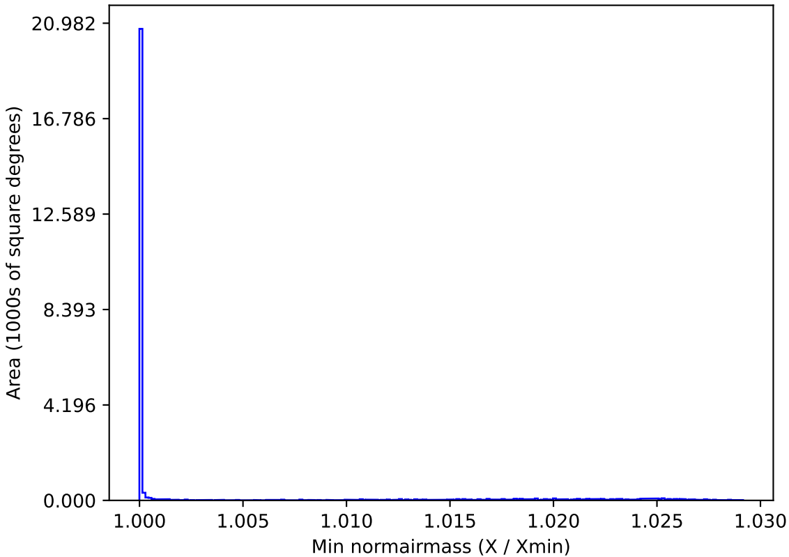
weather_cloudso14v3.4_10yrs All sky all bands: Min normairmass
