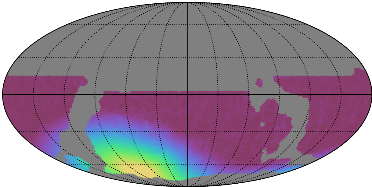
weather_cloudso14v3.4_10yrs WFD z band: Min moonDistance
