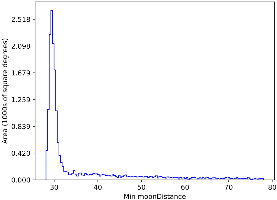
weather_cloudso14v3.4_10yrs WFD z band: Min moonDistance
