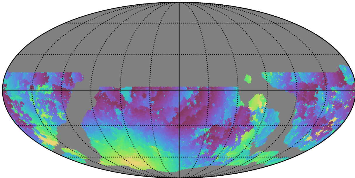
weather_cloudso14v3.4_10yrs WFD u band: Min moonDistance
