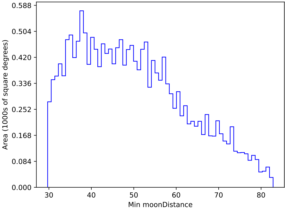
weather_cloudso14v3.4_10yrs WFD u band: Min moonDistance
