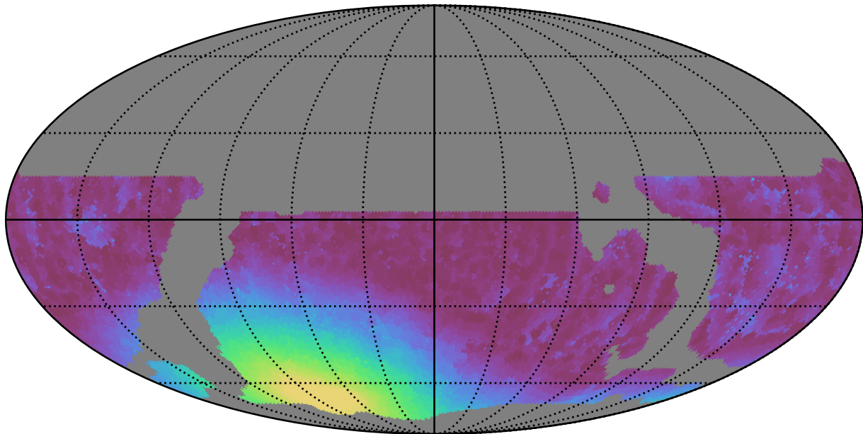
weather_cloudso14v3.4_10yrs WFD r band: Min moonDistance
