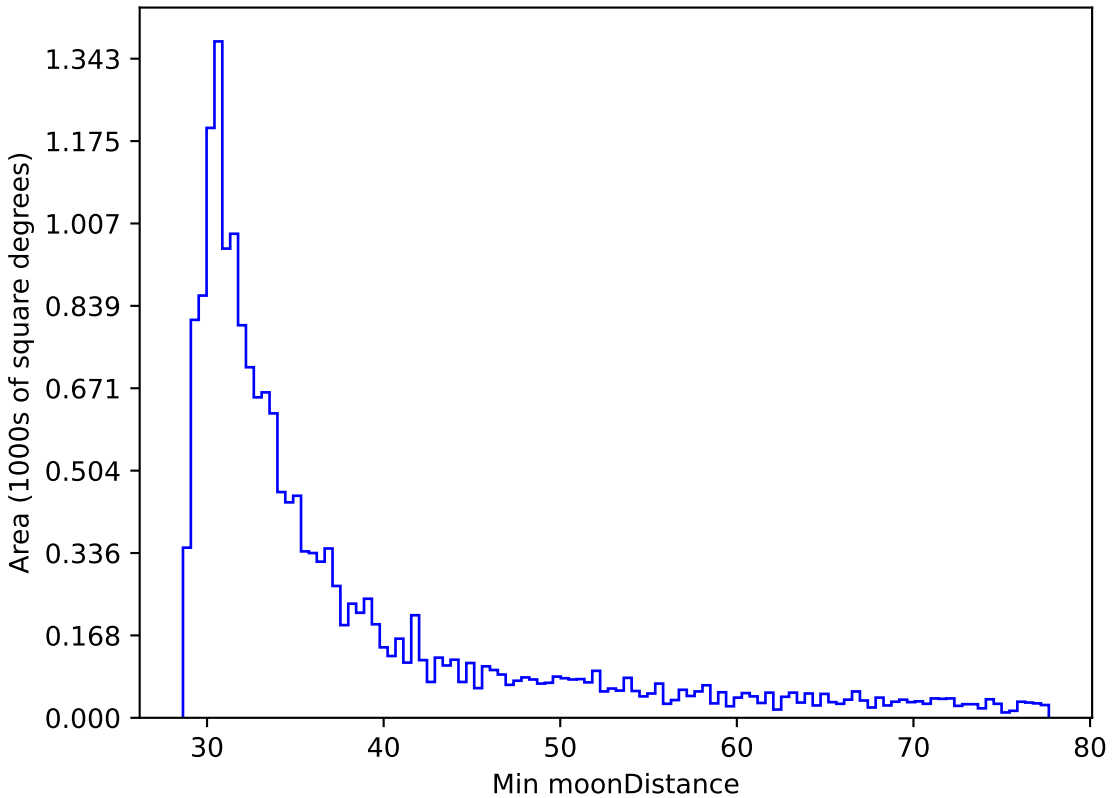
weather_cloudso14v3.4_10yrs WFD r band: Min moonDistance
