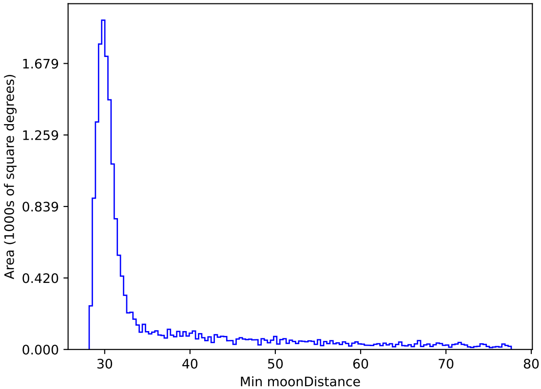
weather_cloudso14v3.4_10yrs WFD i band: Min moonDistance
