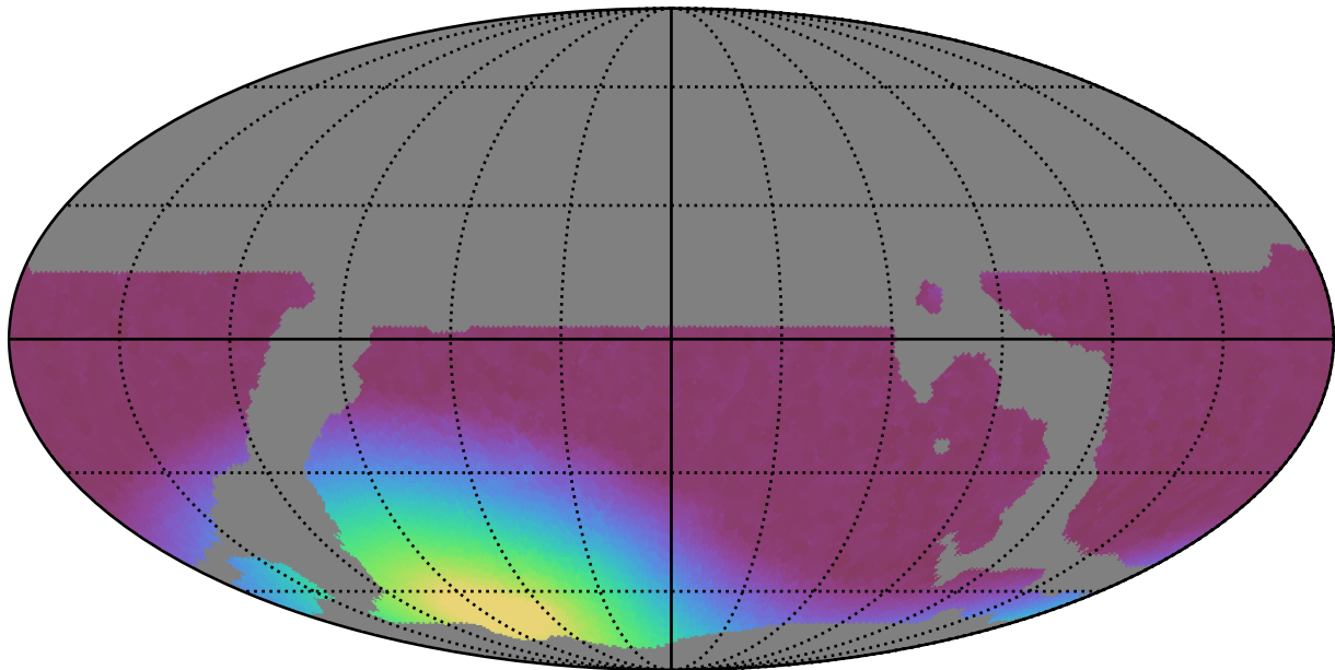
weather_cloudso14v3.4_10yrs WFD all bands: Min moonDistance
