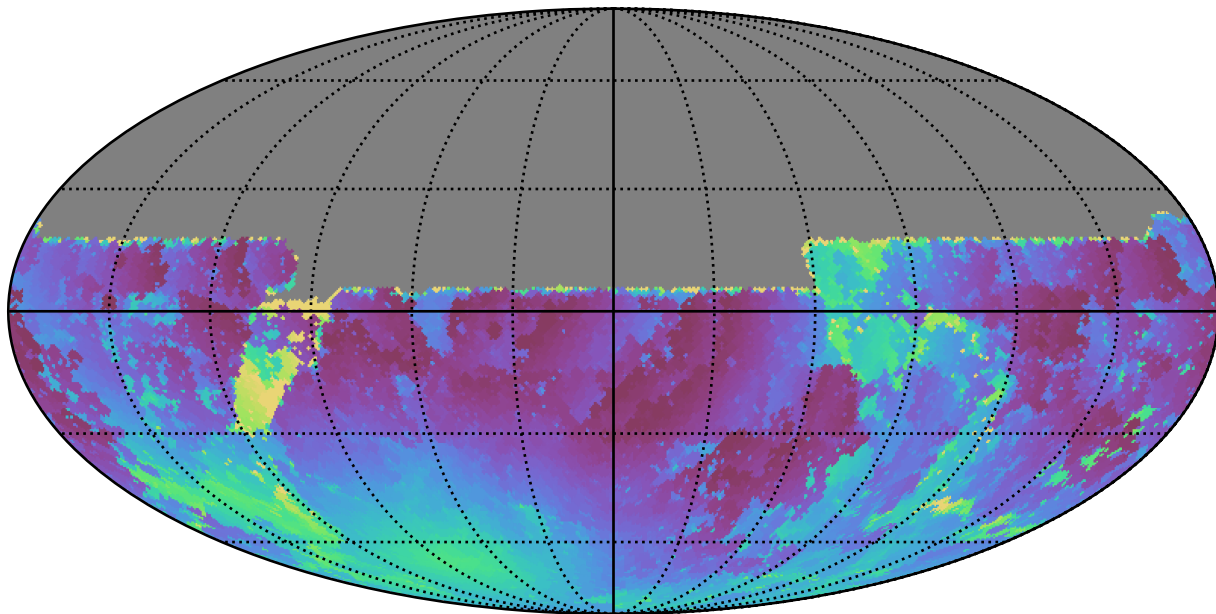
weather_cloudso14v3.4_10yrs All sky u band: Min moonDistance
