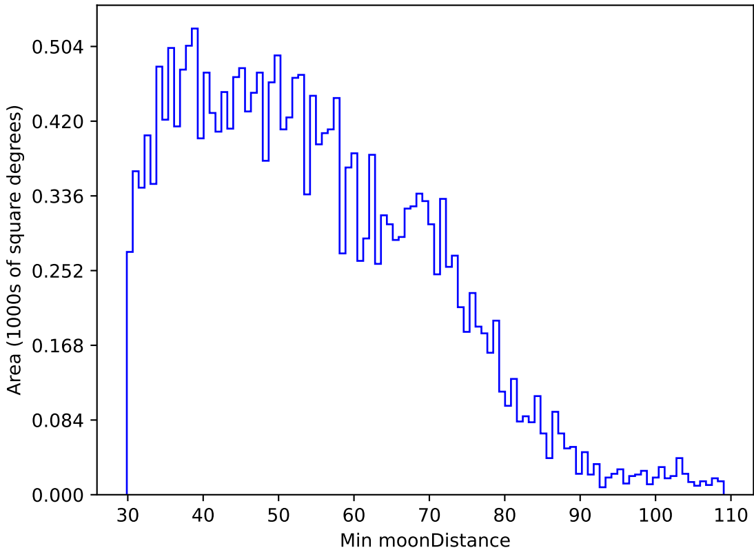
weather_cloudso14v3.4_10yrs All sky u band: Min moonDistance
