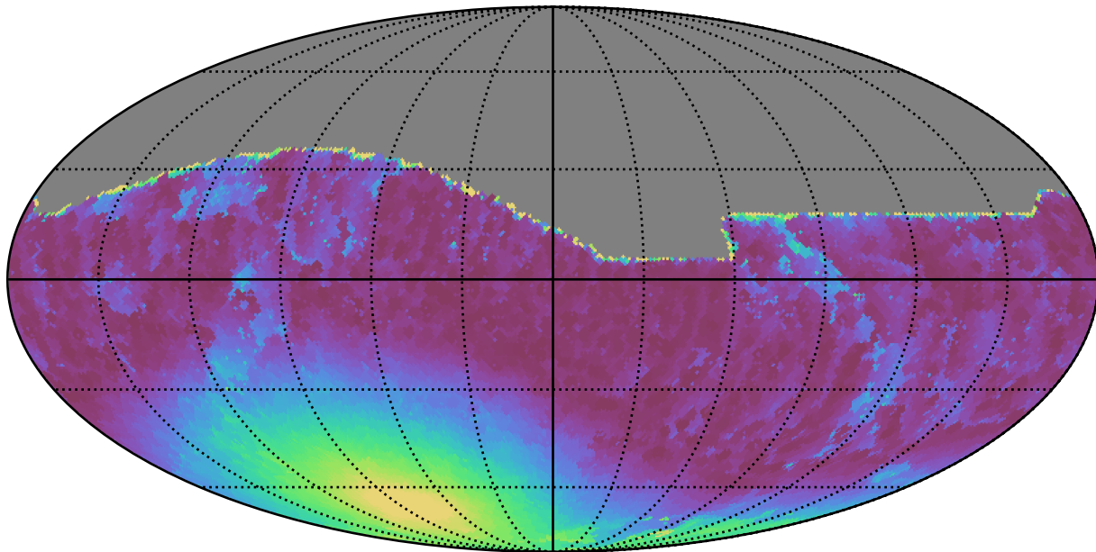
weather_cloudso14v3.4_10yrs All sky r band: Min moonDistance
