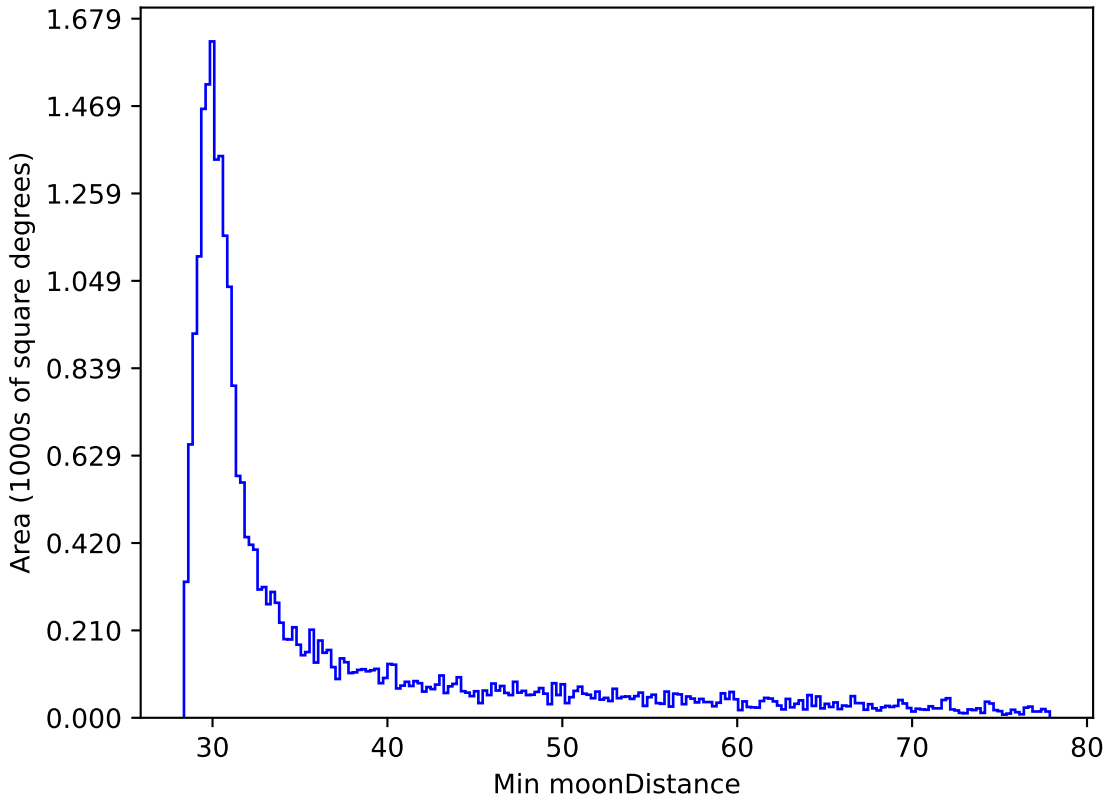
weather_cloudso14v3.4_10yrs All sky i band: Min moonDistance
