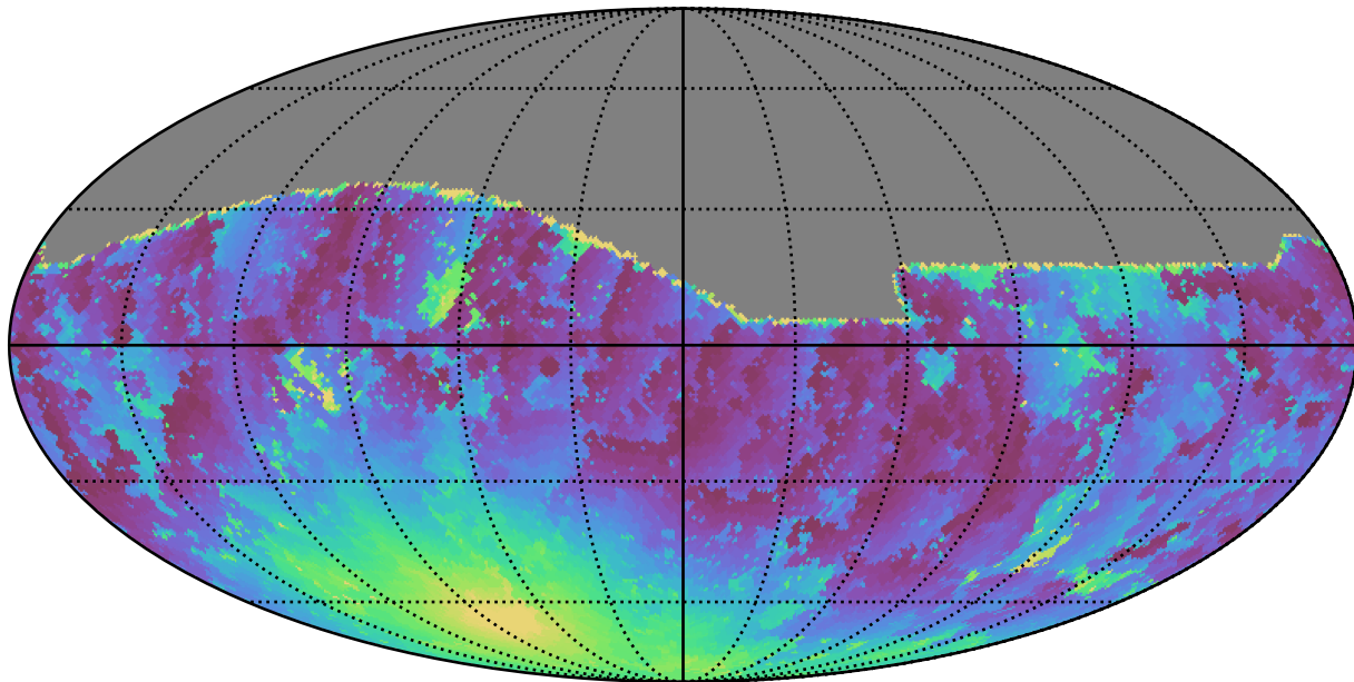
weather_cloudso14v3.4_10yrs All sky g band: Min moonDistance
