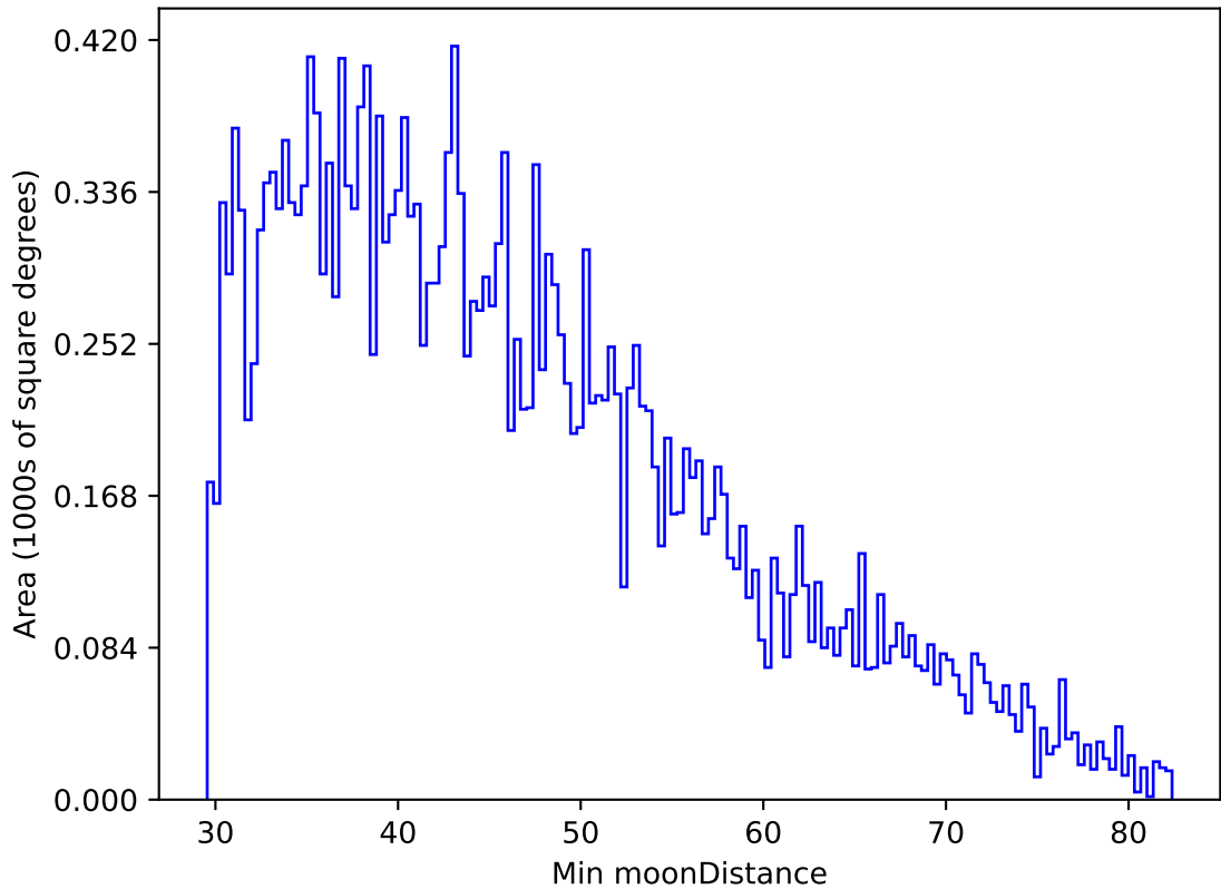
weather_cloudso14v3.4_10yrs All sky g band: Min moonDistance
