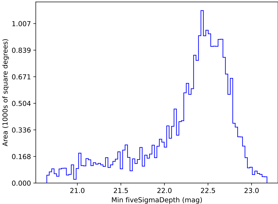
weather_cloudso14v3.4_10yrs Yr 1 z band: Min fiveSigmaDepth
