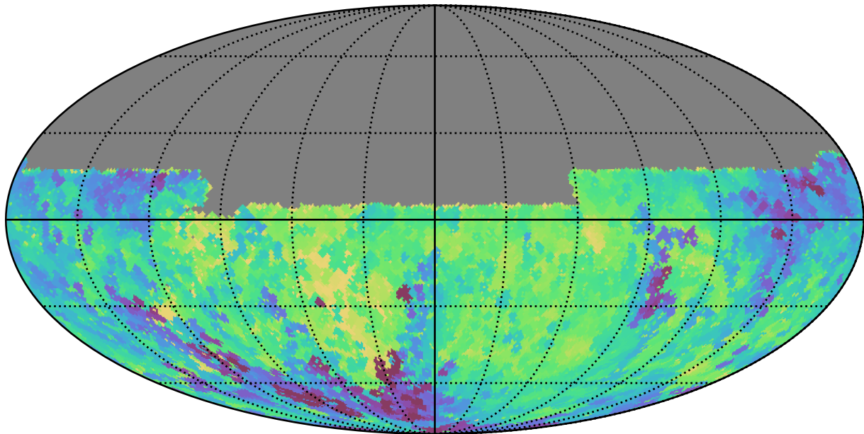
weather_cloudso14v3.4_10yrs Yr 1 y band: Min fiveSigmaDepth
