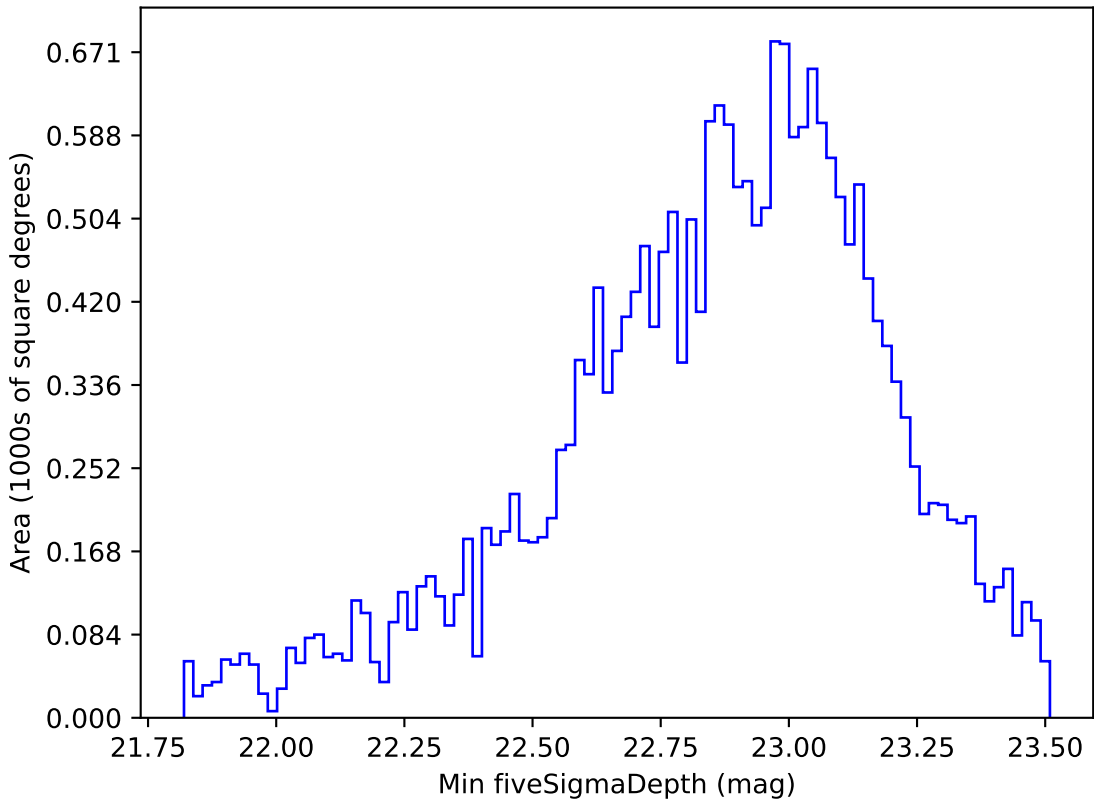
weather_cloudso14v3.4_10yrs Yr 1 u band: Min fiveSigmaDepth
