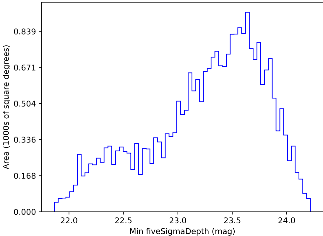
weather_cloudso14v3.4_10yrs Yr 1 r band: Min fiveSigmaDepth
