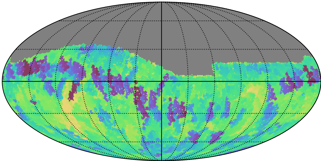
weather_cloudso14v3.4_10yrs Yr 1 i band: Min fiveSigmaDepth
