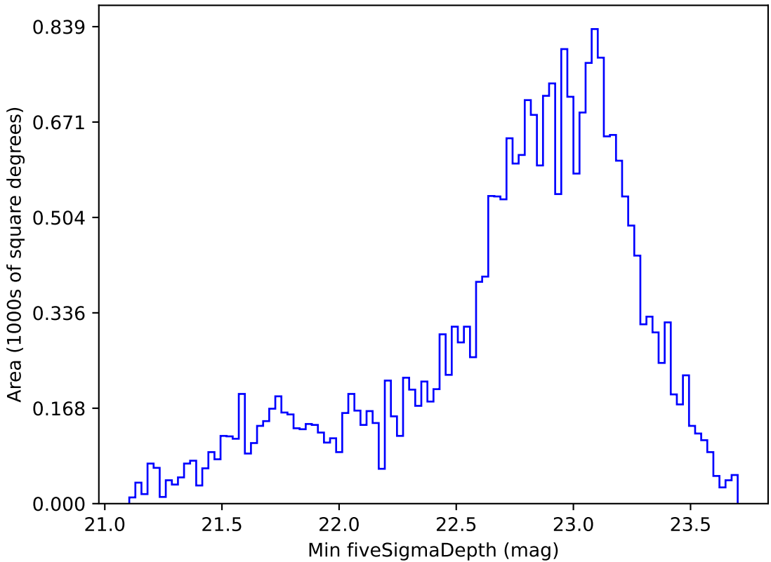
weather_cloudso14v3.4_10yrs Yr 1 i band: Min fiveSigmaDepth
