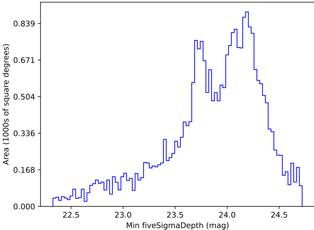
weather_cloudso14v3.4_10yrs Yr 1 g band: Min fiveSigmaDepth
