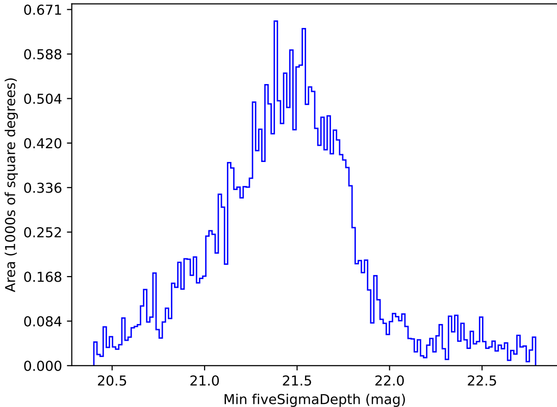
weather_cloudso14v3.4_10yrs Yr 1 all bands: Min fiveSigmaDepth
