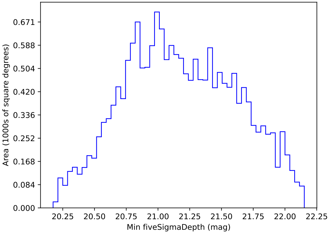
weather_cloudso14v3.4_10yrs WFD z band: Min fiveSigmaDepth
