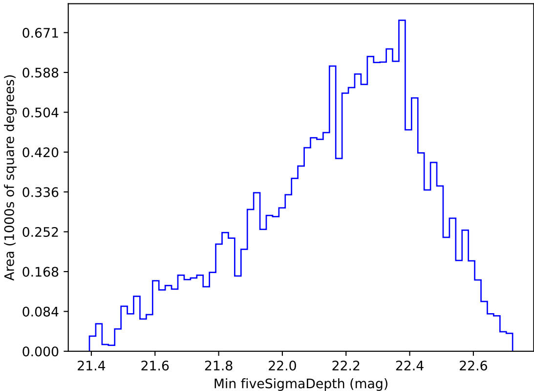
weather_cloudso14v3.4_10yrs WFD u band: Min fiveSigmaDepth
