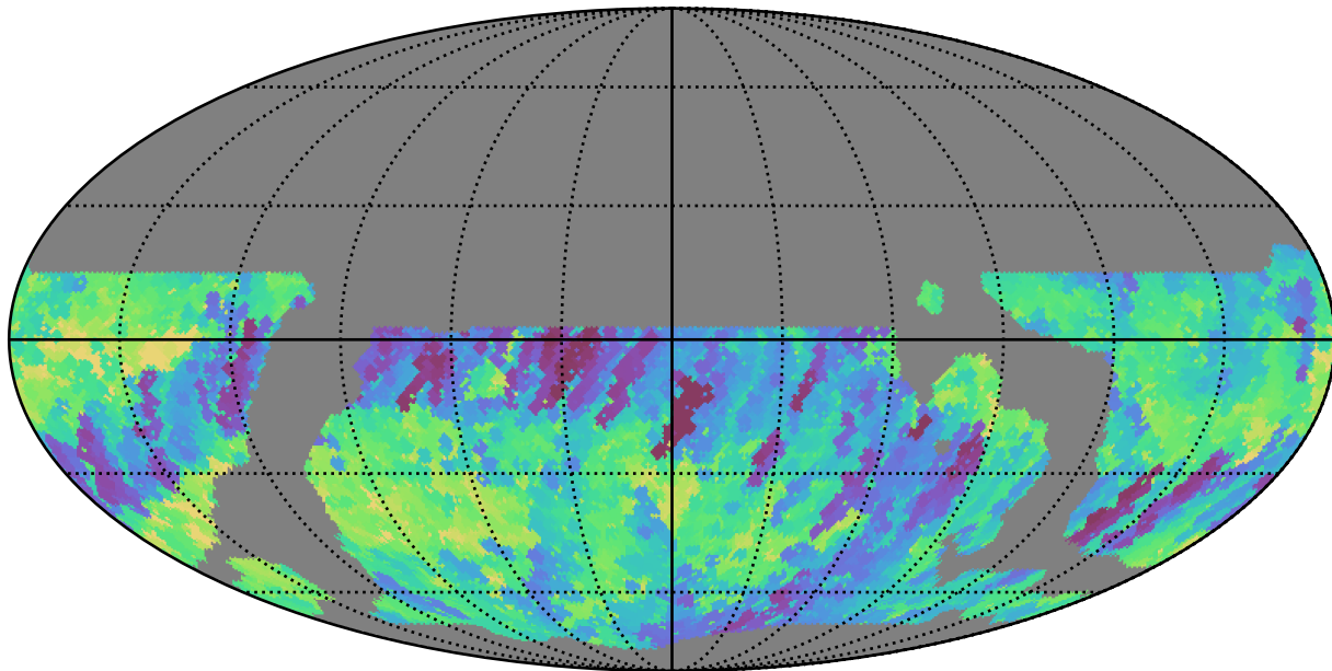
weather_cloudso14v3.4_10yrs WFD r band: Min fiveSigmaDepth
