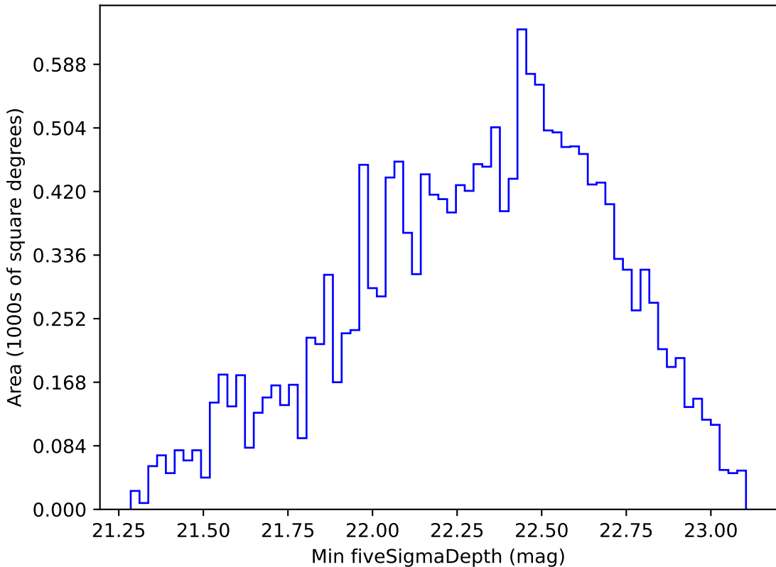
weather_cloudso14v3.4_10yrs WFD r band: Min fiveSigmaDepth
