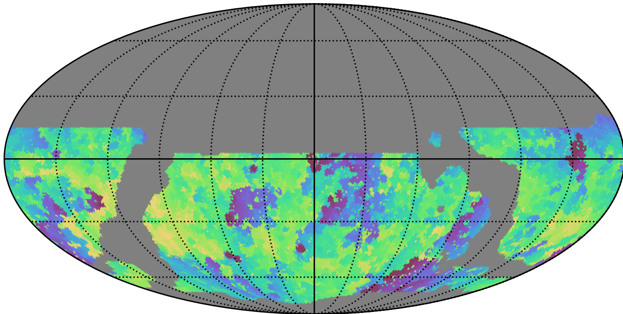
weather_cloudso14v3.4_10yrs WFD g band: Min fiveSigmaDepth
