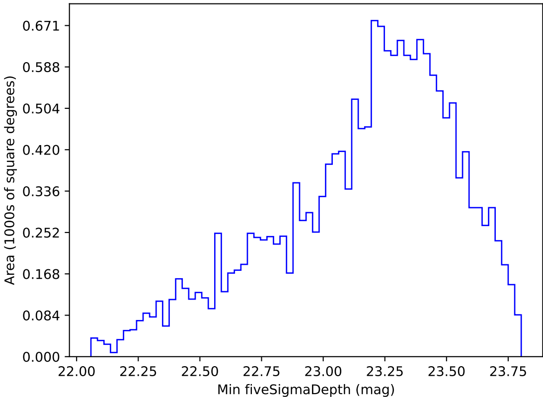
weather_cloudso14v3.4_10yrs WFD g band: Min fiveSigmaDepth
