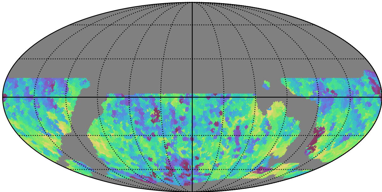
weather_cloudso14v3.4_10yrs WFD all bands: Min fiveSigmaDepth
