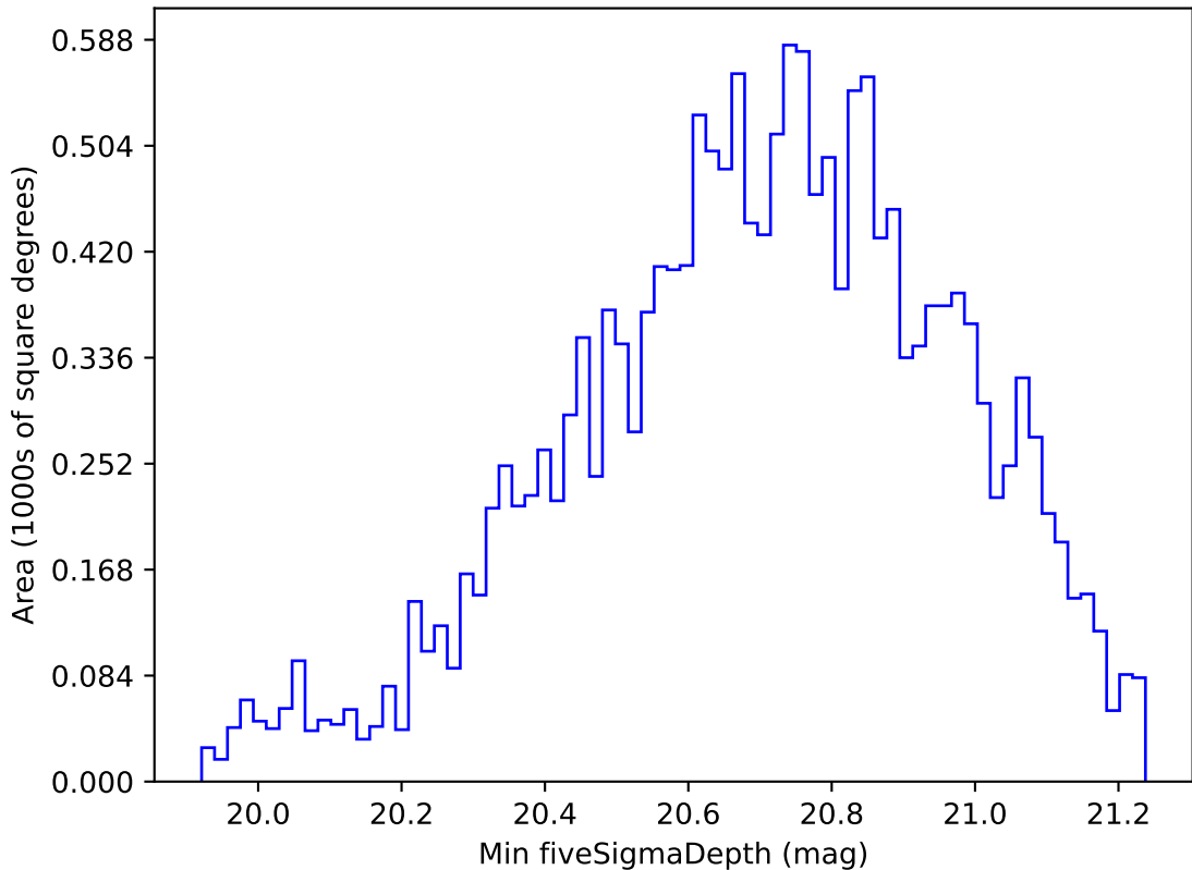
weather_cloudso14v3.4_10yrs WFD all bands: Min fiveSigmaDepth
