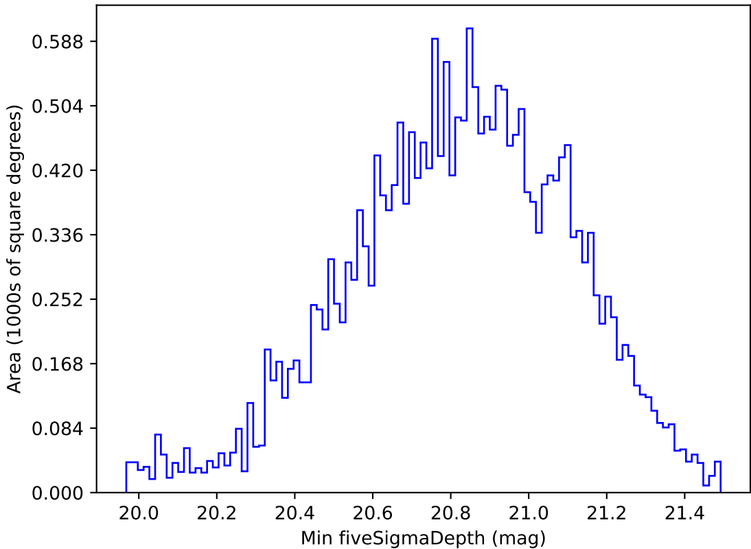
weather_cloudso14v3.4_10yrs All sky y band: Min fiveSigmaDepth
