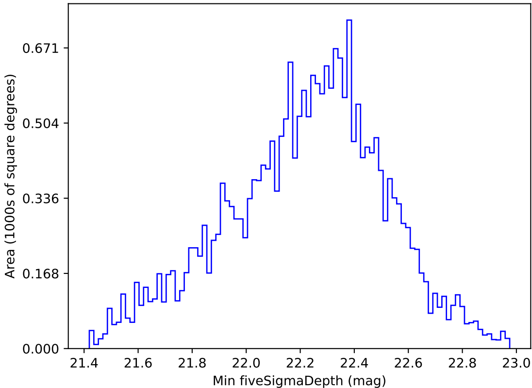
weather_cloudso14v3.4_10yrs All sky u band: Min fiveSigmaDepth
