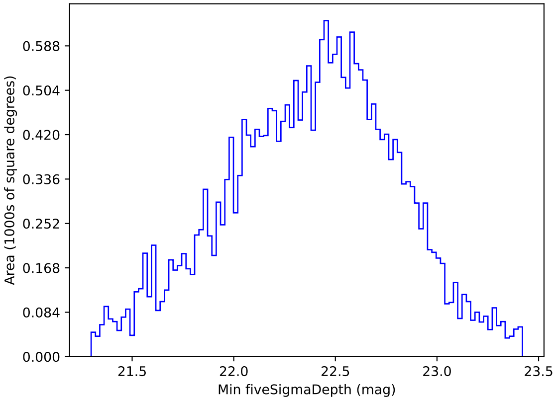
weather_cloudso14v3.4_10yrs All sky r band: Min fiveSigmaDepth
