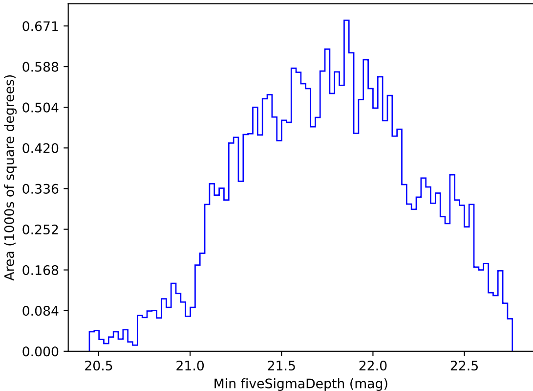
weather_cloudso14v3.4_10yrs All sky i band: Min fiveSigmaDepth
