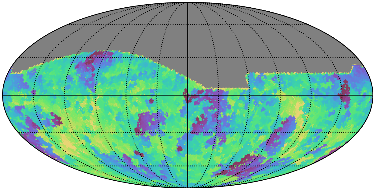
weather_cloudso14v3.4_10yrs All sky g band: Min fiveSigmaDepth
