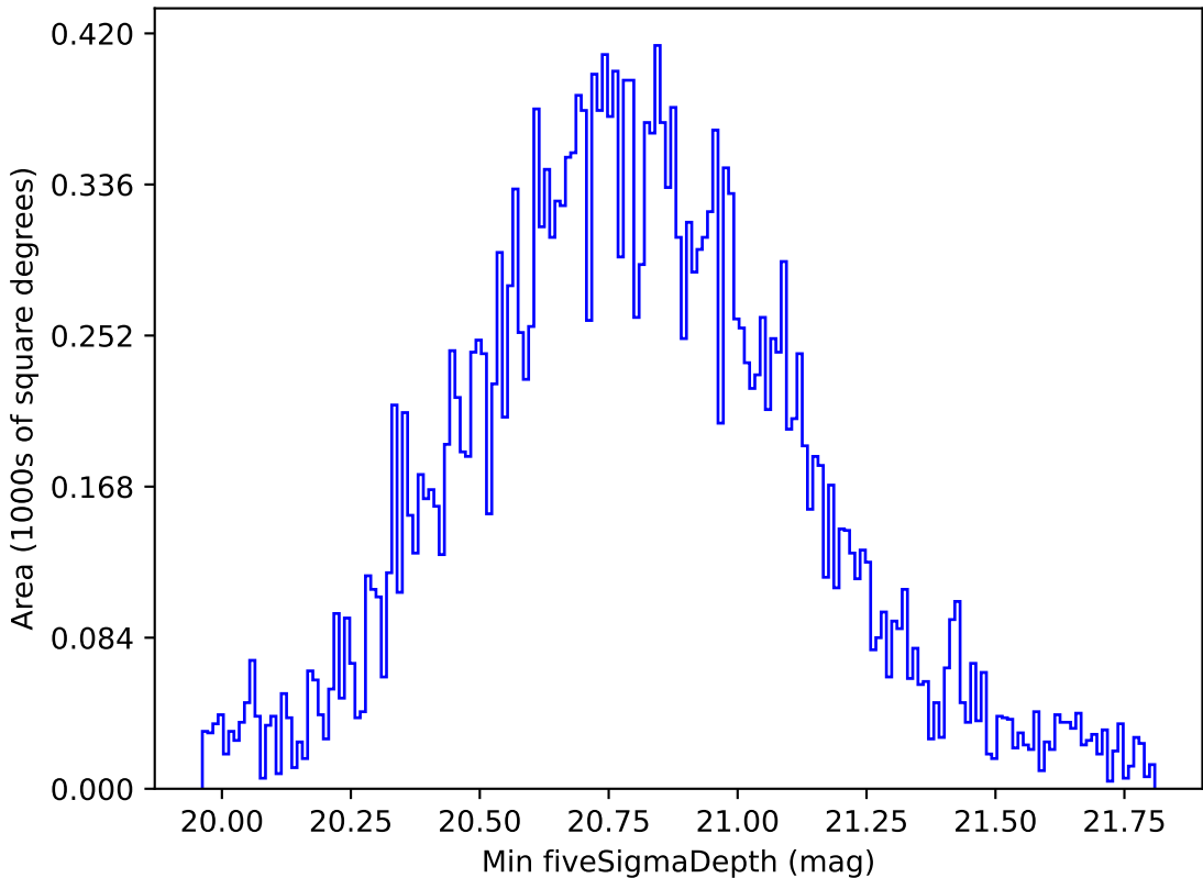
weather_cloudso14v3.4_10yrs All sky all bands: Min fiveSigmaDepth
