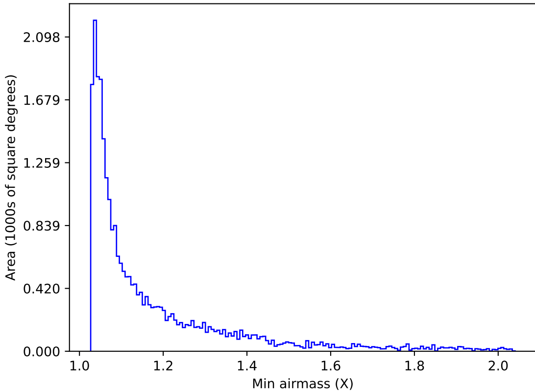
weather_cloudso14v3.4_10yrs Yr 1 z band: Min airmass
