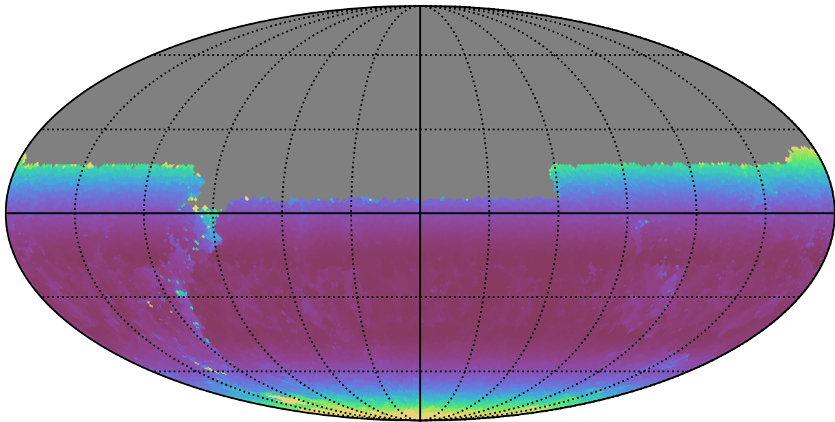
weather_cloudso14v3.4_10yrs Yr 1 y band: Min airmass
