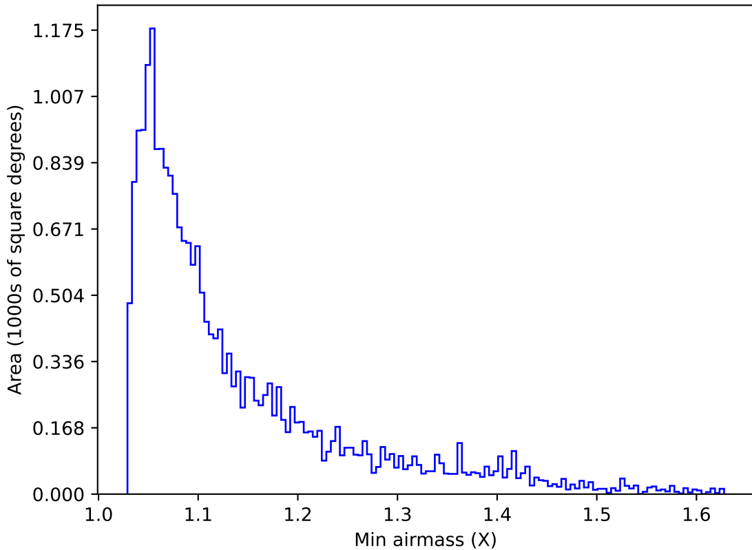
weather_cloudso14v3.4_10yrs Yr 1 u band: Min airmass
