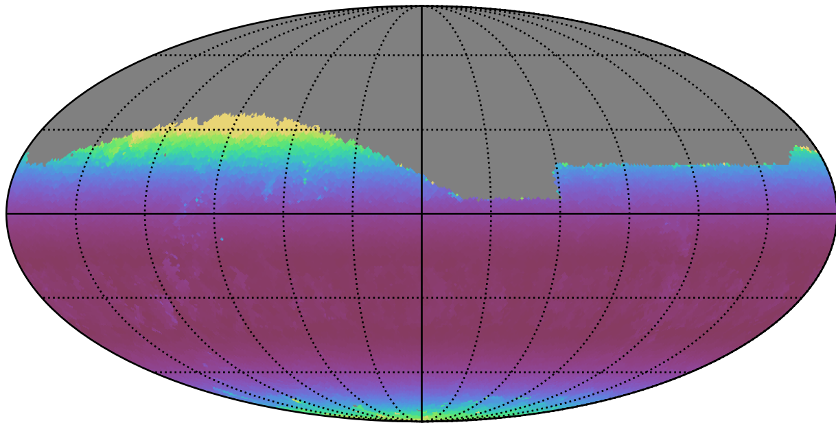
weather_cloudso14v3.4_10yrs Yr 1 r band: Min airmass
