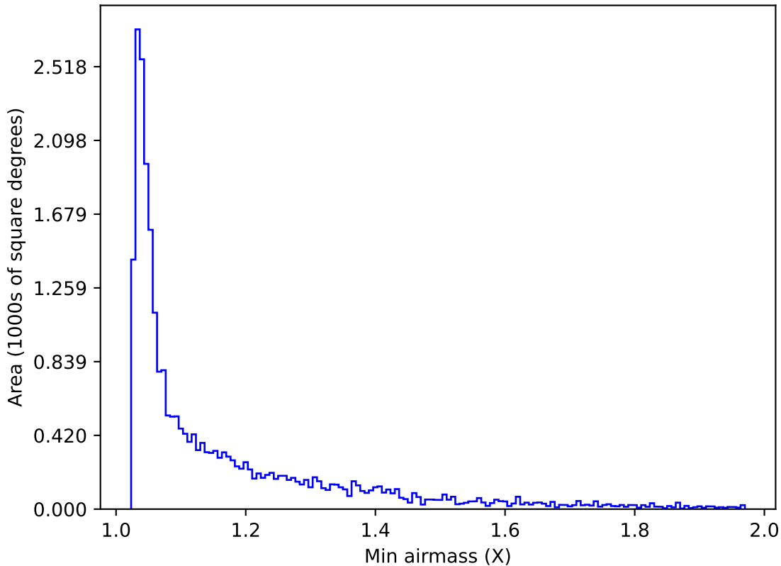
weather_cloudso14v3.4_10yrs Yr 1 r band: Min airmass
